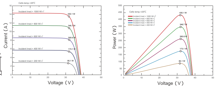
Current-Voltage & Power-Voltage Curves (SKT430M10-108D3)
